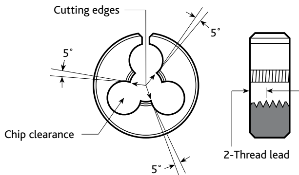
Figure 3 3-Flute die for external threads
