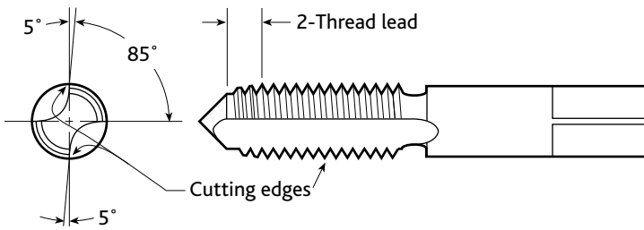
Figure 2 2-Flute tap for internal threads
