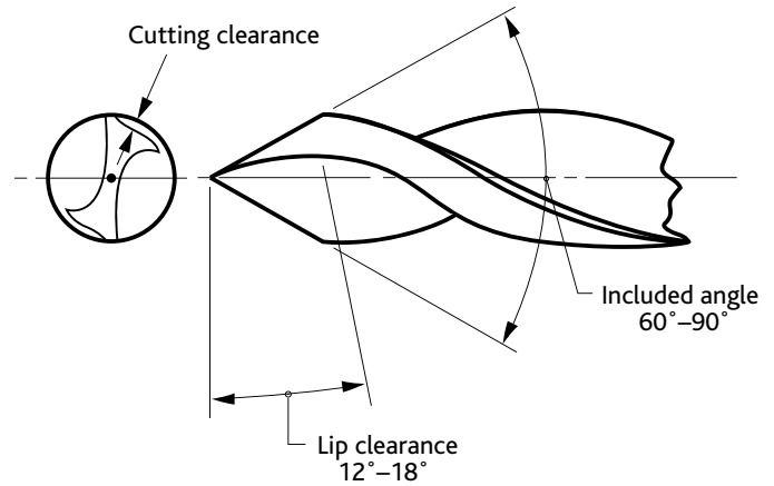
Figure 1 Suggested drill-point design for drilling cellulosic plastic
