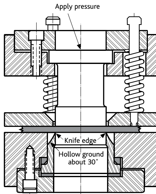
Figure 5 Blanking and Punching Assembly
