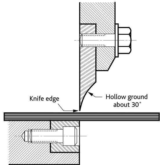
Figure 4 Shearing Assembly
